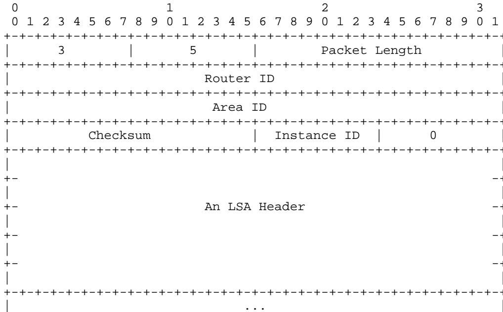
The OSPF Link State Acknowledgment Packet
