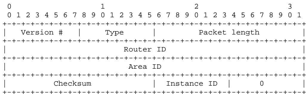
The OSPF Packet Header
