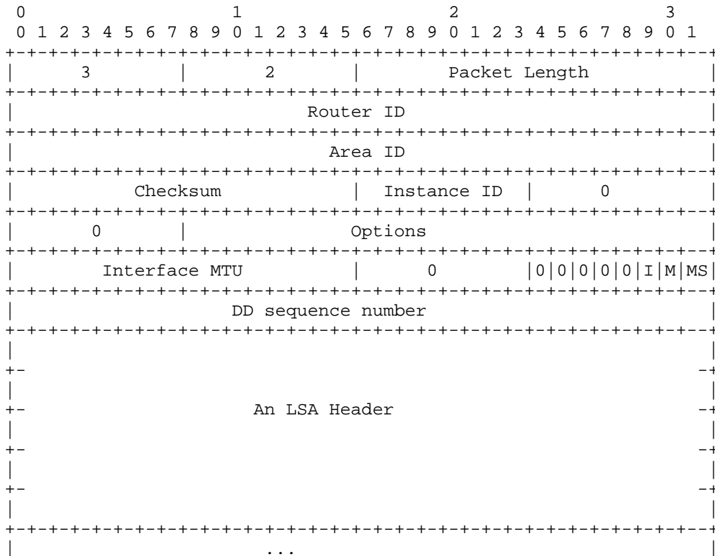
The OSPF Database Description Packet
