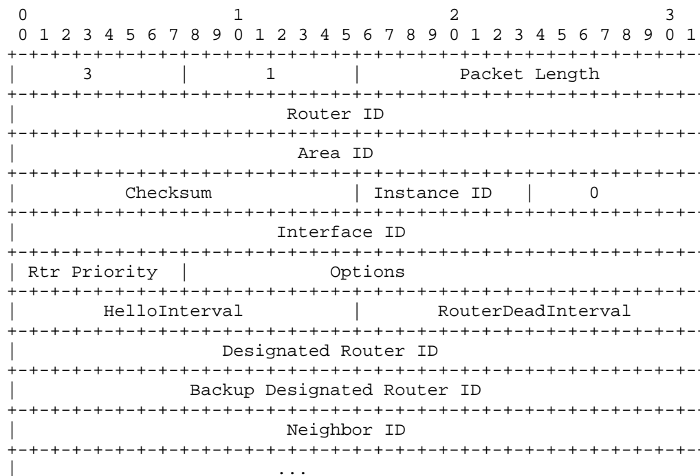
The OSPF Hello Packet
