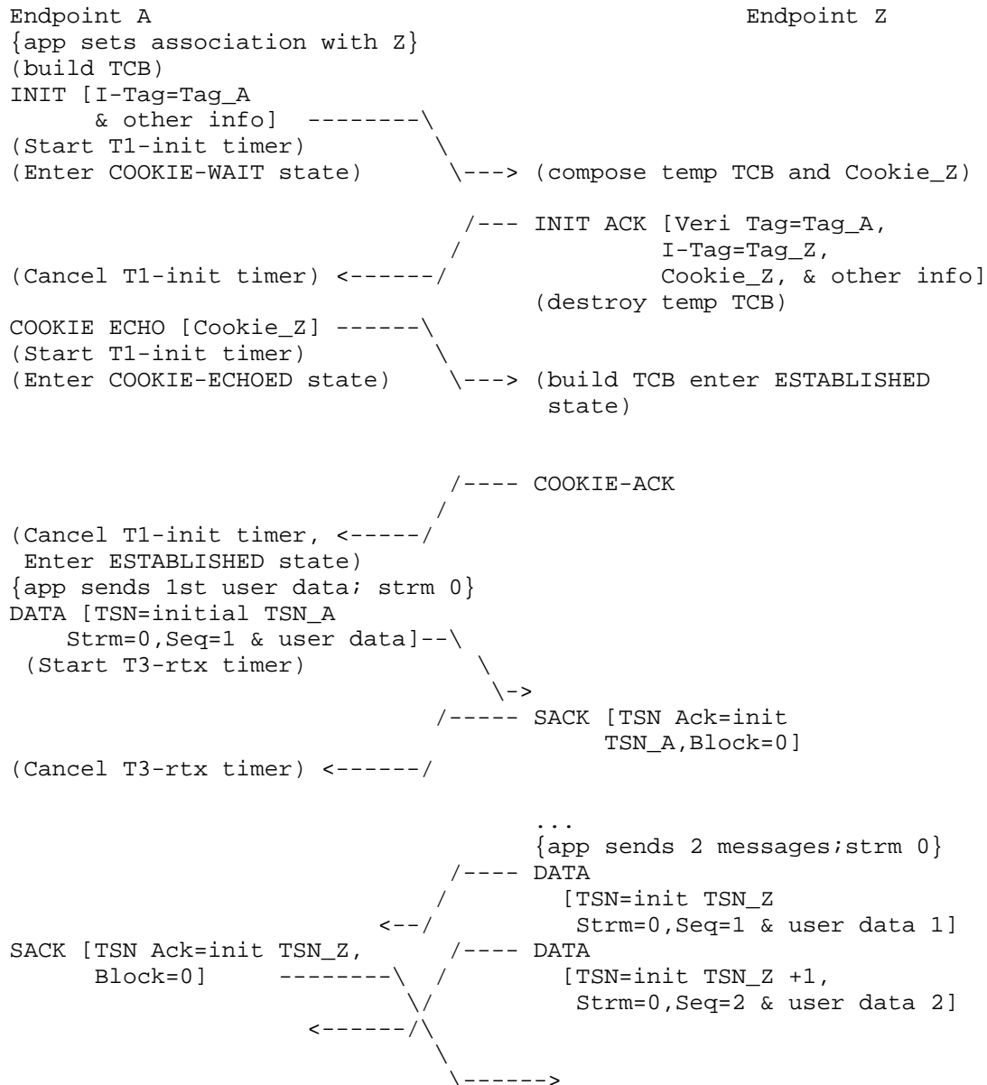
Figure 4: INITiation Example
