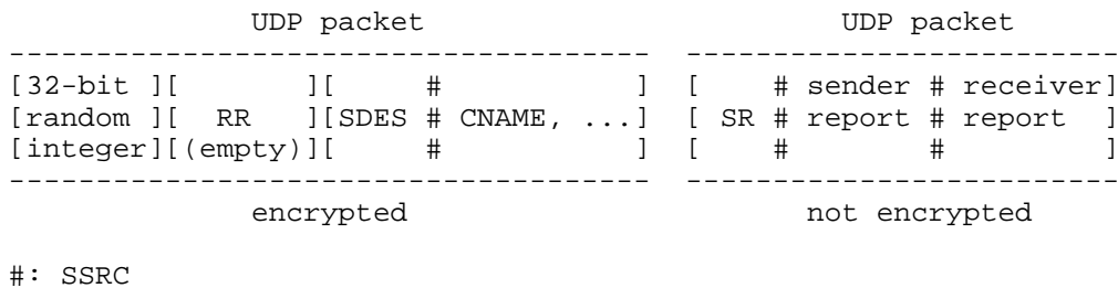
Figure 4: Encrypted and non-encrypted RTCP packets
