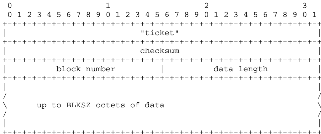
Fig. 4: Data Packet
