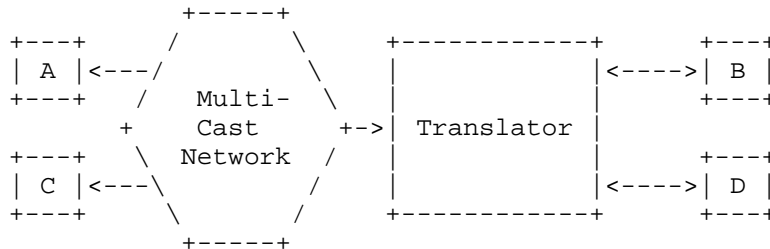
Figure 3 - Point to Multipoint Using a Translator
