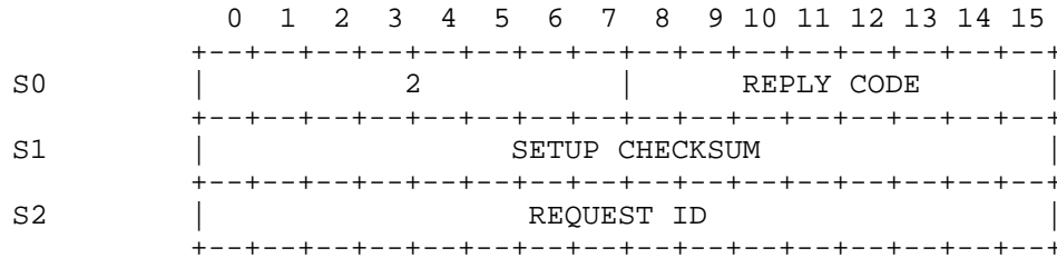
ADD GROUP MEMBER REPLY Figure 22
