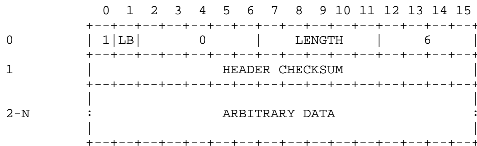
NO OPERATION (NOP) Figure 41
