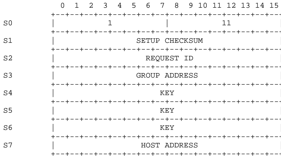
REMOVE GROUP MEMBER REQUEST Figure 25
