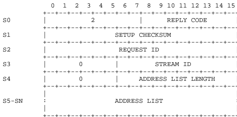
CREATE STREAM REPLY Figure 9
