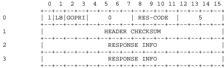
UNNUMBERED RESPONSE Figure 5
