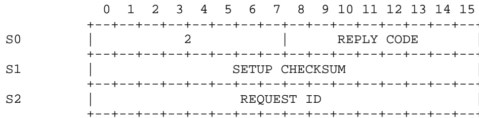
DELETE GROUP REPLY Figure 28
