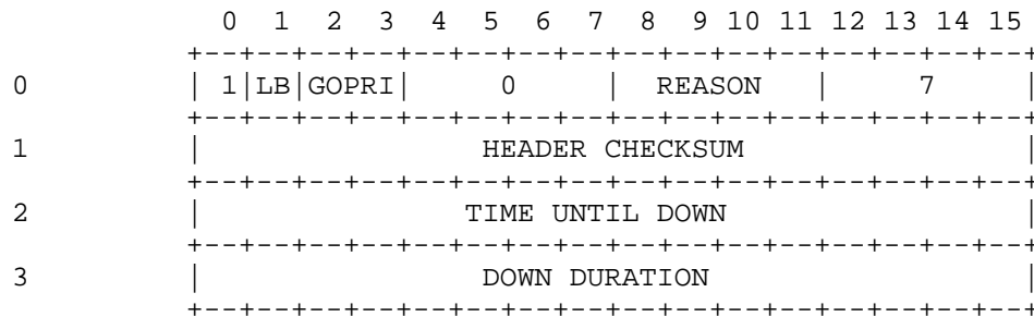
LINK GOING DOWN Figure 40
