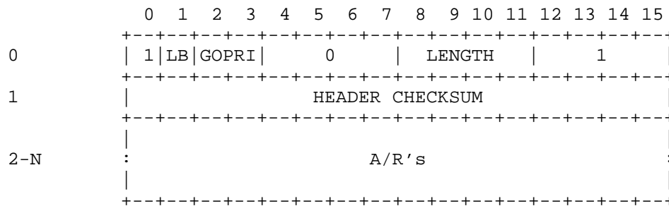
ACCEPTANCE/REFUSAL MESSAGE Figure 4
