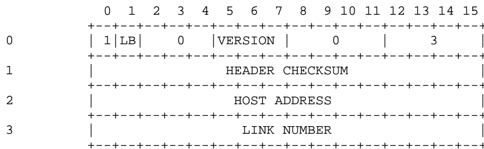
RESTART REQUEST Figure 37
