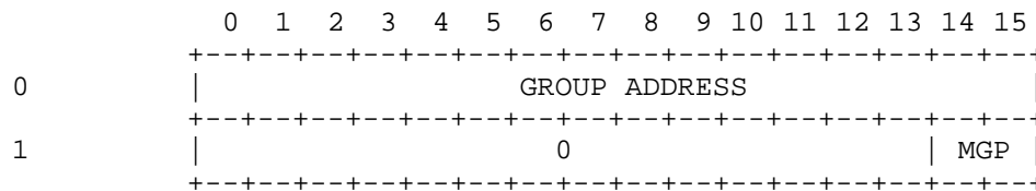
GROUP INFORMATION Figure 34
